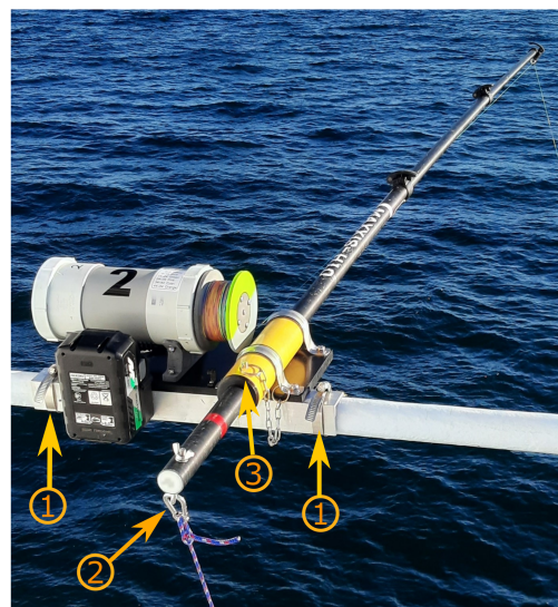
Figure 1. Winch unit installed on a ship's railing showing hose clamps, securing pin, and attachment carabiner.
